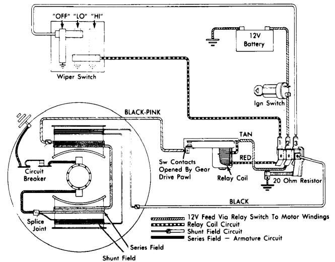
General Motors Round Motor Wiper System Wiring Diagram
