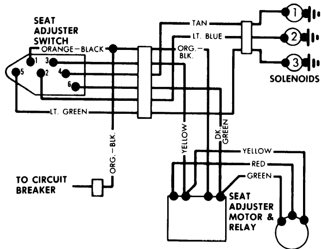
General Motors 6-Way Electric Seat Control Wiring Diagram
