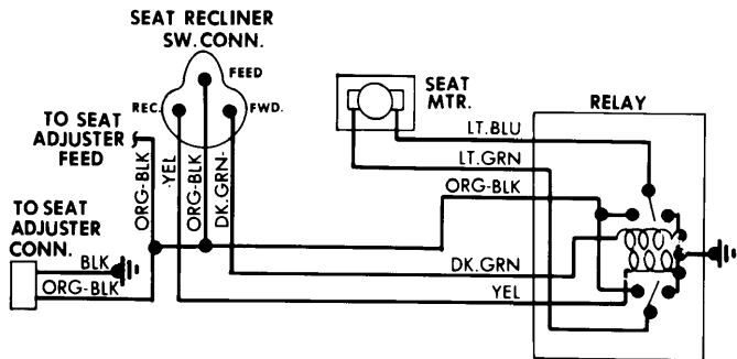
General Motors Reclining Seat Back Wiring Diagram
